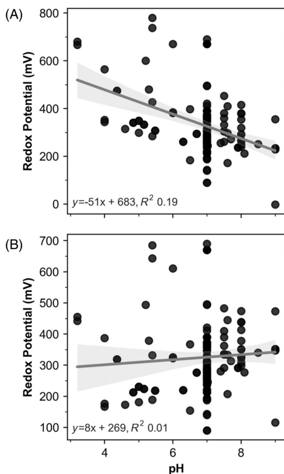
FIGURE 3 Cu cofactor type correlation of pH and redox potential (A) experimental results and (B) normalized using the Nernst equation (Equation (1)). Figures include linear regression with a 95% confidence interval and the equation of best fit.
