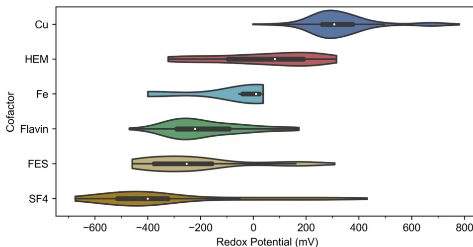
FIGURE 1 Distribution of redox potentials for the most abundant cofactor types found in ProtRedox. Sorted according to mean redox potential cofactors and displayed vertically from most reducing to most oxidizing along with corresponding atomic structures. SF4 (4Fe4S; 82) -329 \pm 268 mV; FES (2Fe2S; 64) -220 \pm 199 mV; Flavin (114) -183 \pm 141 mV; Fe (10) -72 \pm 173 mV; HEM (42) 43 \pm 190 mV; Cu (147) 333 \pm 129 mV. Count of each cofactor type is within parenthesis.
