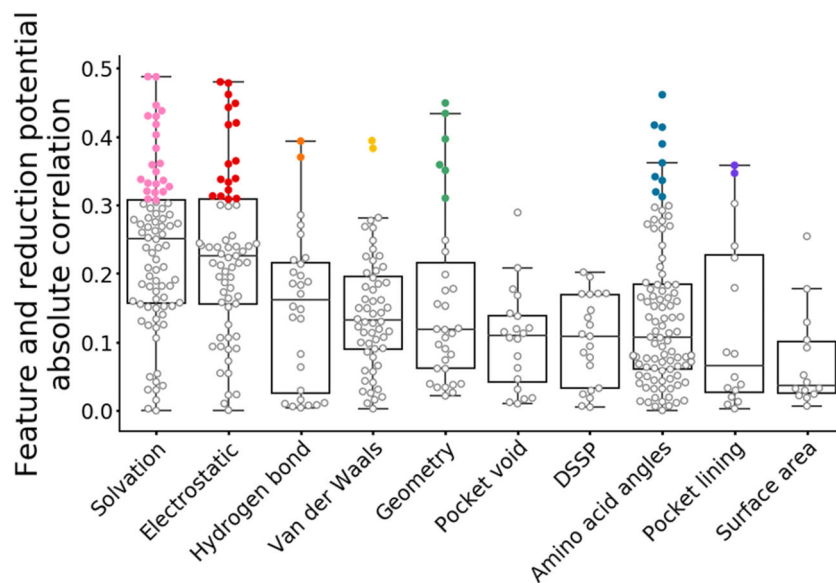
FIGURE 2 Correlation of reduction potential and physicochemical properties: Groups of physicochemical properties of metalloenzymes that can be measured from protein structure are shown along the x-axis. Each circle is the absolute value of the Pearson correlation coefficient for reduction potentials. Colored circles represent p -value \leq 0.05 for the correlation and empty circles represent p -value \geq 0.05 . Horizontal box lines, from top to bottom, represent the upper quartile, median, and lower quartile correlation values for the respective property category. The whiskers display the range of correlation values for the respective property category, except for outliers, which are greater than 150% of the interquartile range from the box.
